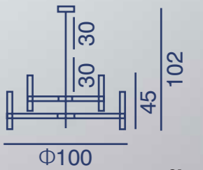
MD80556-30-1000 Φ100x102CM G9x30
