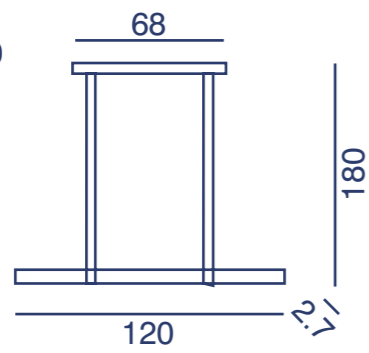
MD80613-1L1200 121x2.7x180CM LED 43W
