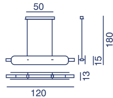
MD21955-2L-1200 120x13x180CM LED 37W
