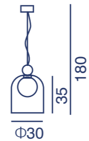
MD80596-1-300 Φ30x180CM LED 9W
