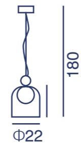
MD80596-1-220 Φ22x180CM LED 9W
